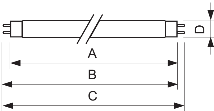
MASTER TL-D Power Saver Set 37=58W/840 1SL
